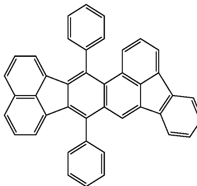
9,16-Diphenylacenaphtho[1,2-k]benzo[e]acephenanthrene
